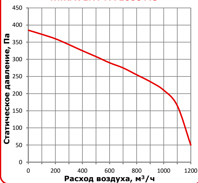
MIRAVENT PA 1000 AC
