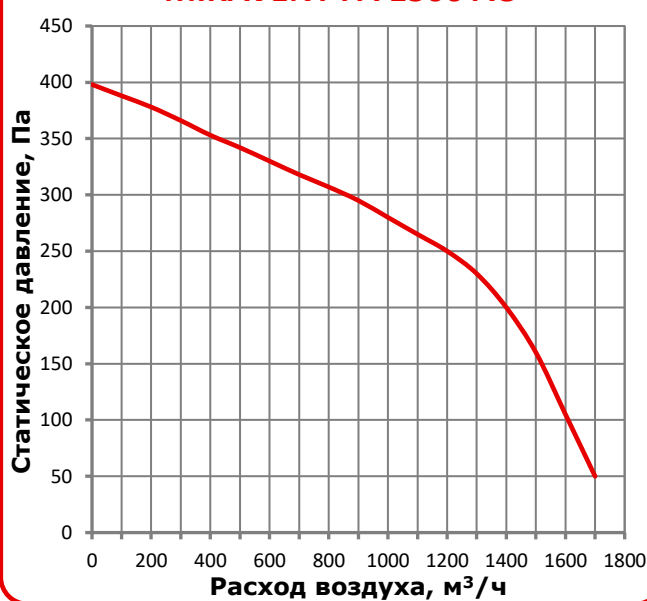
MIRAVENT PA 1500 AC
