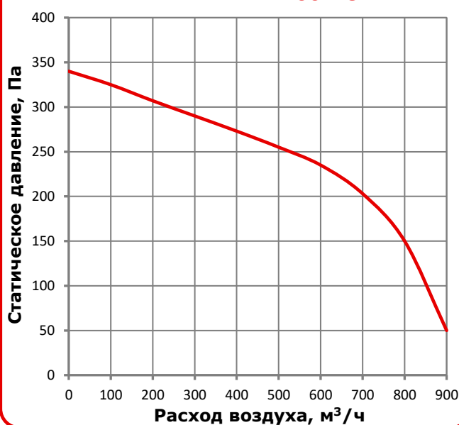
MIRAVENT PA 700 AC
